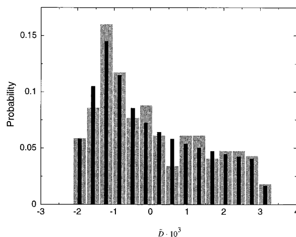
Figure 1. Experimental DC histogram (broad bars) fitted by a ‘powder pattern’ function (narrow bars; see text and Appendix). Experimental data comprise 443 one-bond N-H N , CO-N, and C \alpha -CO couplings from the structured regions of MBP. The fitted parameters are A_a = 1.55 \times 10^{-3} , R = 0.19 (Table 1). A fixed number of histogram bins, 15, over the entire range of normalized dipolar couplings \bar{D}_{IM} have been used throughout these analyses; similar results are obtained with a larger number of bins.
