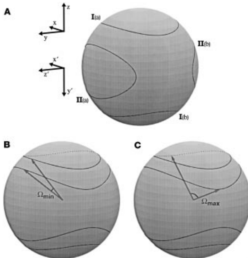
Figure 2. Possible orientations of internuclear vectors corresponding to constant DC values represented by contours on the surface of a unit sphere. The classification of the contours into types I and II is described in the text. Axes x , y , and z represent the principal axes of the alignment tensor. \Omega_{\min} and \Omega_{\max} are the minimum and maximum angles, respectively, between the two internuclear vectors tracing out the pair of contours (DC isolines).
