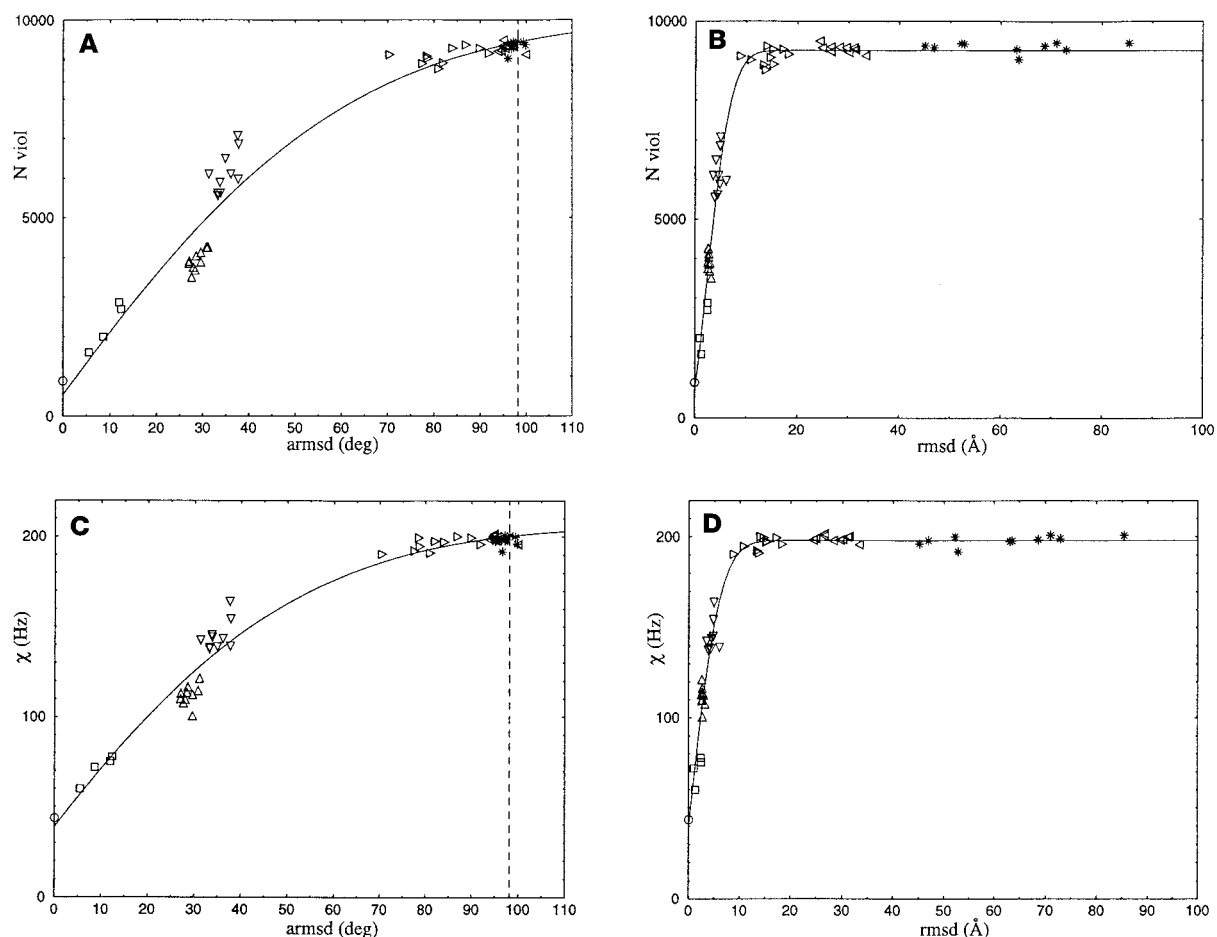
Figure 3. Two penalty functions, N_{\text{viol}} and \chi , calculated on the basis of the experimental dipolar couplings for various MBP structures plotted as a function of angular root mean square deviation (armsd) and root mean square deviation (rmsd) of the structures with respect to 1OMP(S). Armsd is defined as the root mean square of the angle between the internuclear vectors from the trial structure and their counterparts from the reference structure, as computed for the set of N-H N , CO-N, and C α -CO vectors used in generating Figure 1. The symbols in the plot represent: (●) structure 1OMP(S); (■) X-ray crystallography structures 1OMP (Sharff et al., 1992), 1DMB (Sharff et al., 1993), 1ANF (Quioco et al., 1997), and 4MBP (Quioco et al., 1997); (▲) set of NMR structures based on NOE, dihedral angle, chemical shift, and DC restraints including 1943 amide-amide, amide-methyl, and methyl-methyl NOE restraints (Mueller et al., 2000); (▼) NMR structures based on NOE, dihedral angle, and chemical shift restraints; (►) NMR structures based on partial NOE data (729 amide-amide NOE restraints); (◄) structures obtained via partial thermal unfolding of the NOE-based structures using the program CNS (Brünger et al., 1998); (*) random conformers with the primary sequence of MBP generated using the program TRADES (Feldman and Hogue, 2000) and refined using the program CNS. The parameter N_{\text{viol}} was calculated using the set of experimental DC data consisting of one-bond N-H N , CO-N, and C α -CO couplings from the structured regions in MBP. The solid lines in each of the plots help guide the eye. The dashed line indicates the limiting value of armsd, as defined in the text, for a pair of unrelated structures with uniformly distributed orientations of the internuclear vectors. The values A_a = 1.55 \times 10^{-3} and R = 0.19 have been used in these calculations (see Table 1).
